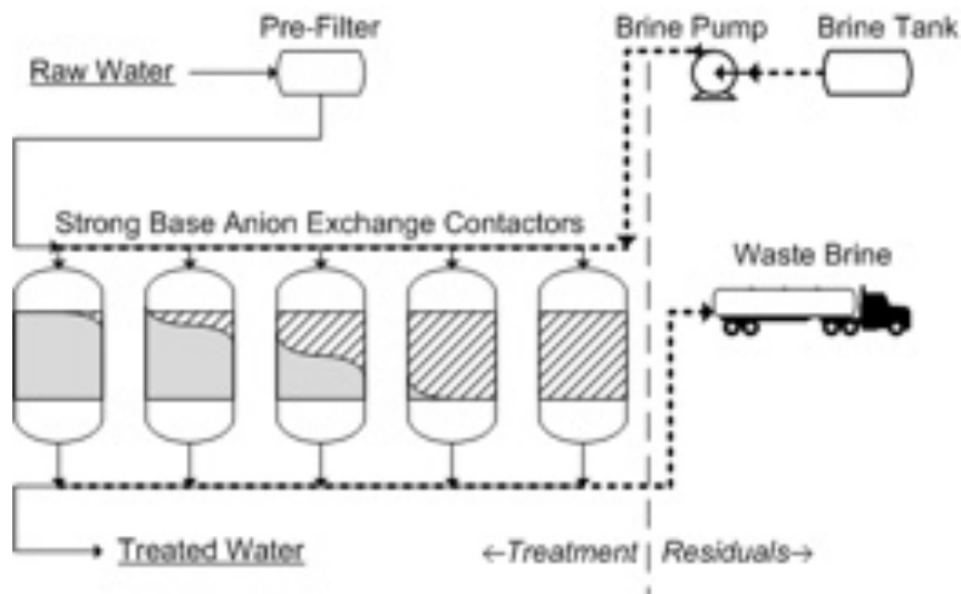
Figure 5. Typical SBA-IX treatment process schematic.
