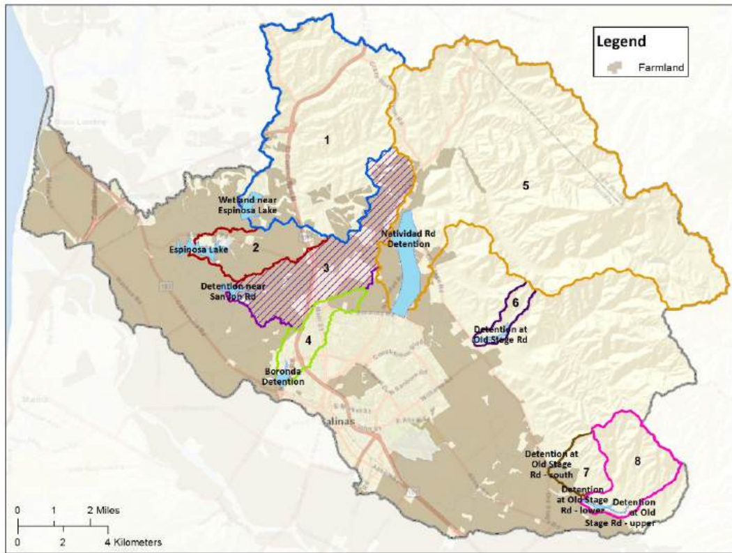
Figure 6.11a The Ten Gabilan Sub-Watershed Basins in the Nitrate Box Model (# 1 – 8)
